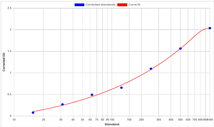
Standard curve Infliximab ELISA Kit 62000 [ng/mL]
