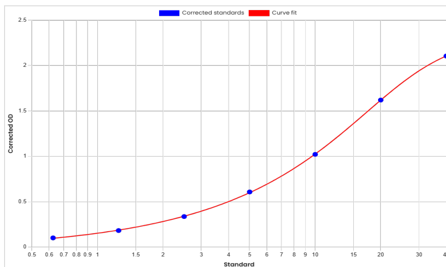
Standard curve Rabbit anti-PEG IgG ELISA Kit 60822 [ng/mL]
