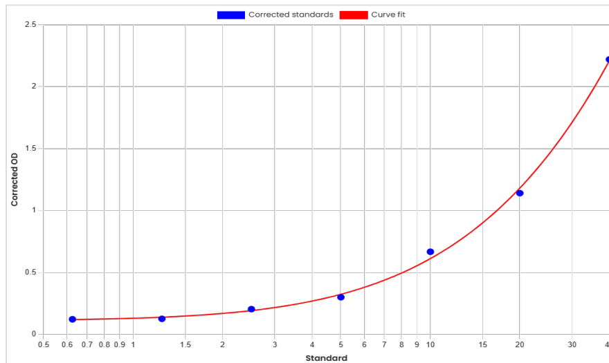
Standard curve T-Dxd ELISA 60792 [ng/mL]
