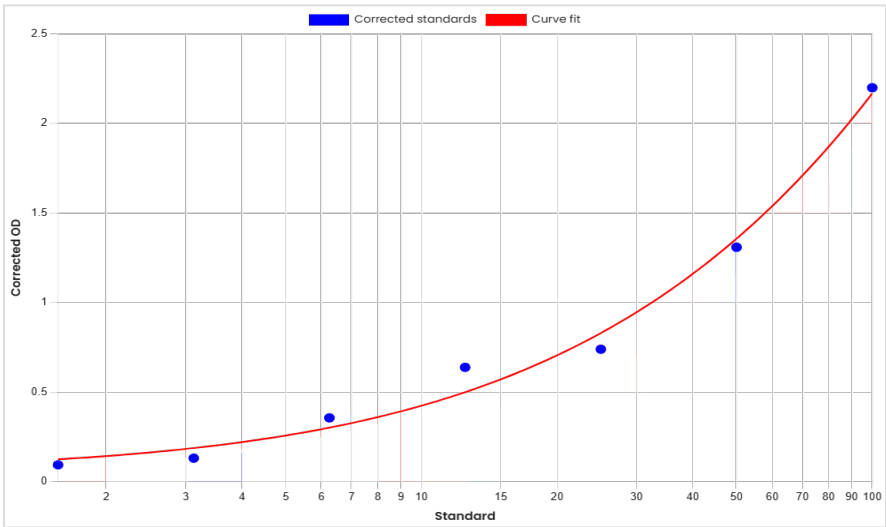
Standard curve anti-Zilovertamab vedotin antibodies (ADA) ELISA 60775 [ng/mL]
