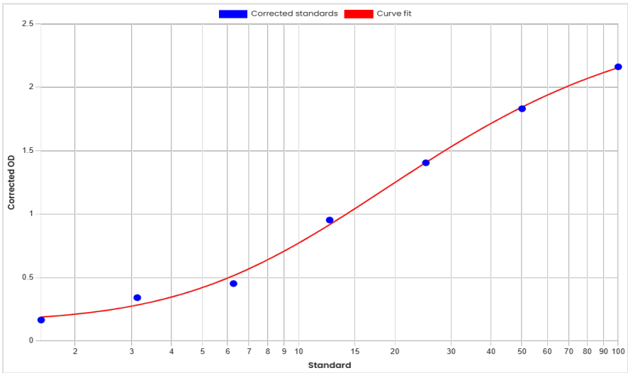
Standard curve anti-Epcoritamab antibodies (ADA) ELISA 60758 [ng/mL]
