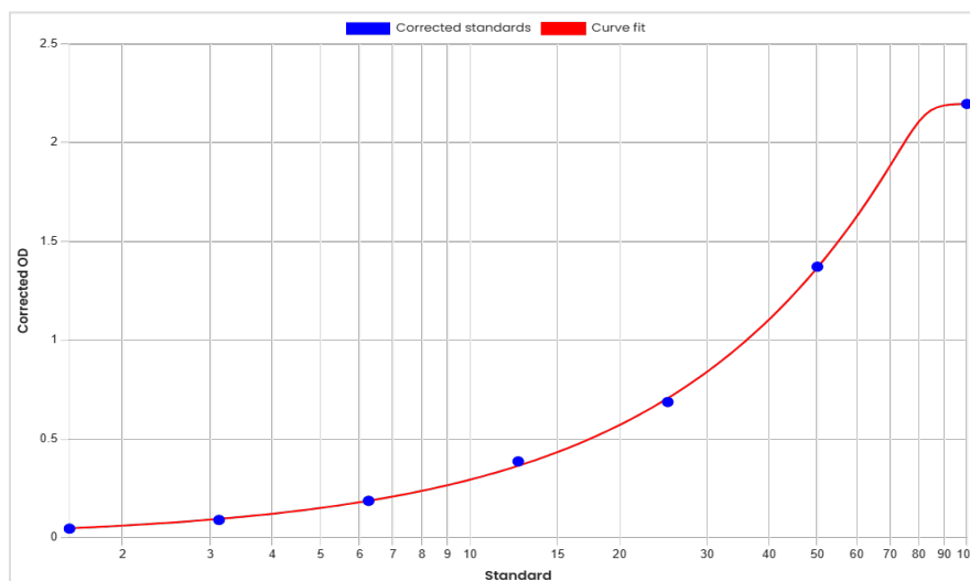
Standard curve anti-Inezetamab antibodies (ADA) ELISA 60755 [ng/mL]
