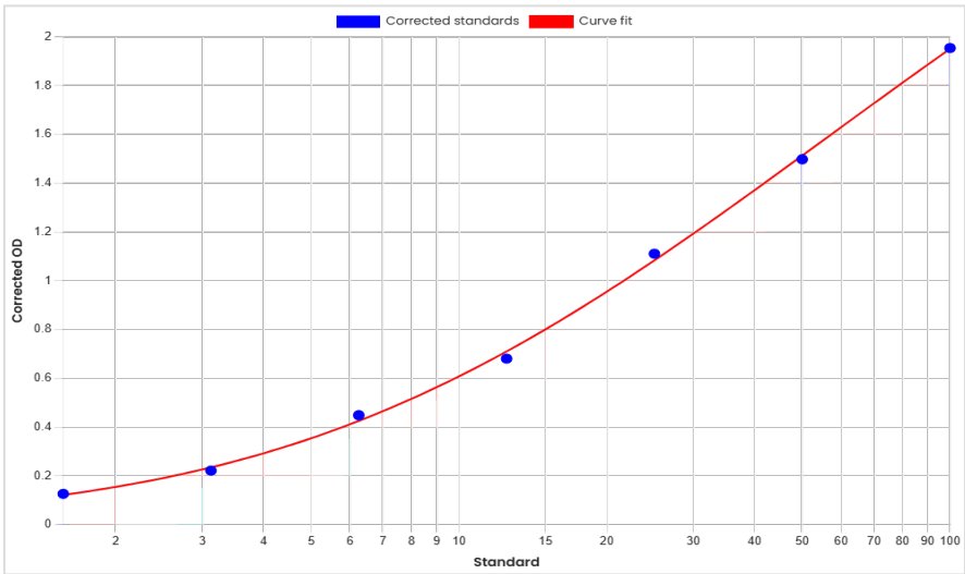
Standard curve anti-Selicrelumab antibodies (ADA) ELISA 60750 [ng/mL]
