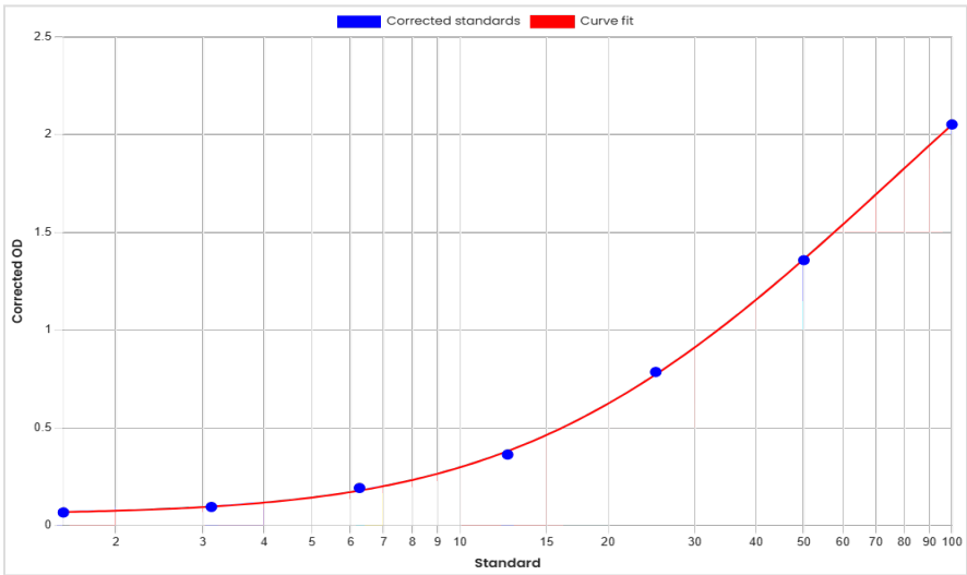
Standard curve anti-Sutimlimab antibodies (ADA) ELISA 60737 [ng/mL]
