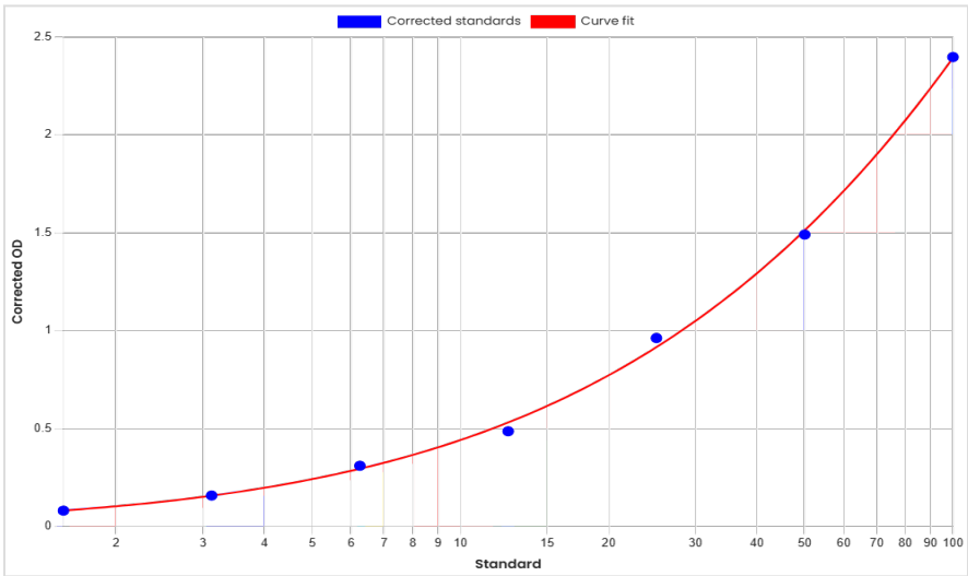
Standard curve anti-Bavituximab antibodies (ADA) ELISA 60711 [ng/mL]
