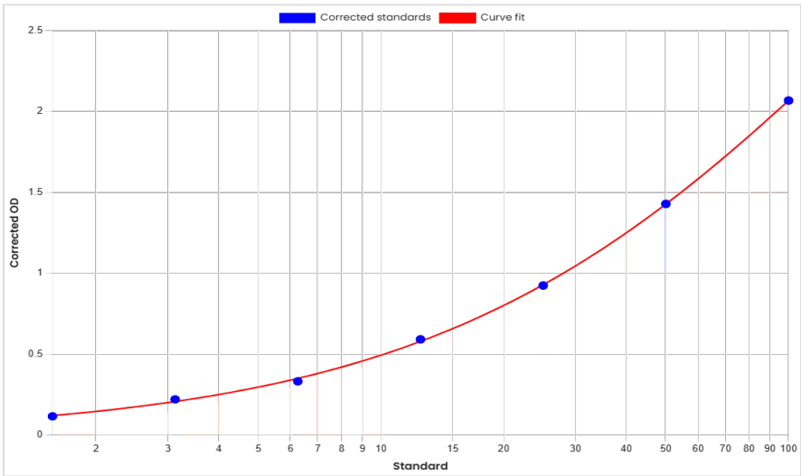
Standard curve anti-Sonepcizumab antibodies (ADA) ELISA 60703 [ng/mL]
