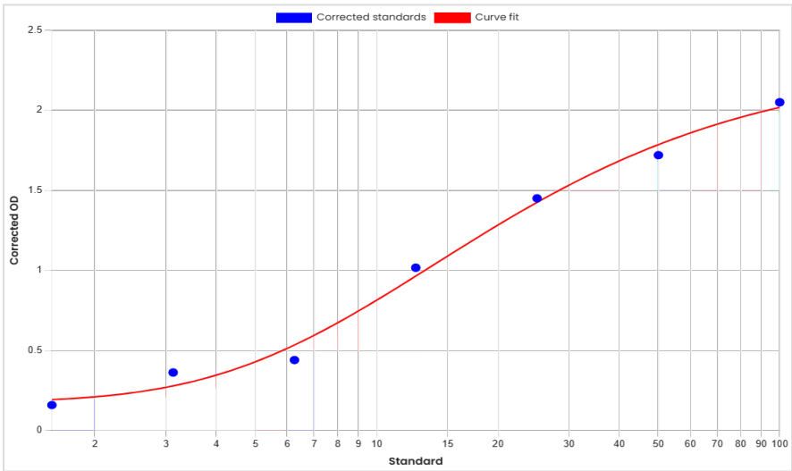
Standard curve anti-Brontictuzumab antibodies (ADA) ELISA 60700 [ng/mL]
