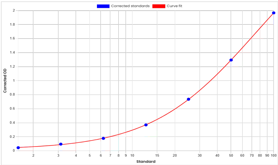
Standard curve anti-Bapotulimab antibodies (ADA) ELISA 60691 [ng/mL]
