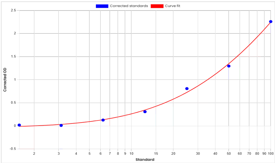
Standard curve anti-Narsoplimab antibodies (ADA) ELISA 60683 [ng/mL]
