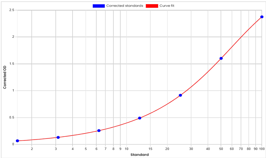
Standard curve anti-Coprelotamab antibodies (ADA) ELISA 60597 [ng/mL]
