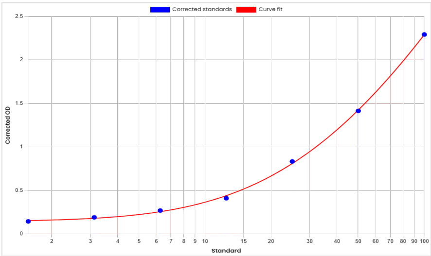
Standard curve anti-Miptenalimab antibodies (ADA) ELISA 60585 [ng/mL]
