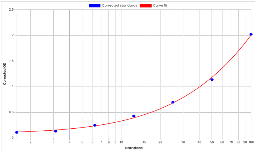
Standard curve anti-3F6-9G5 antibodies (ADA) ELISA 60564 [ng/mL]
