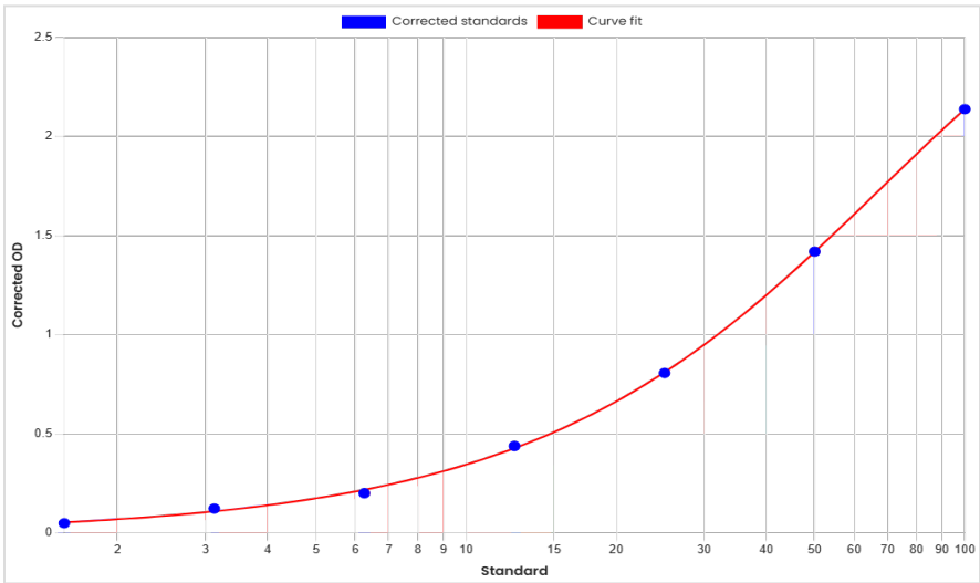
Standard curve anti-Tadocizumab antibodies (ADA) ELISA 60549 [ng/mL]
