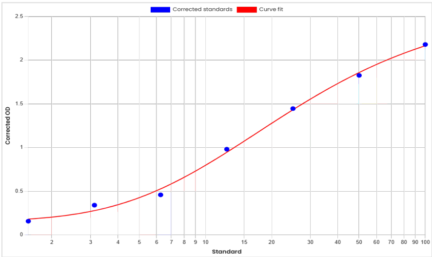
Standard curve anti-Lodapolimab antibodies (ADA) ELISA 60513 [ng/mL]
