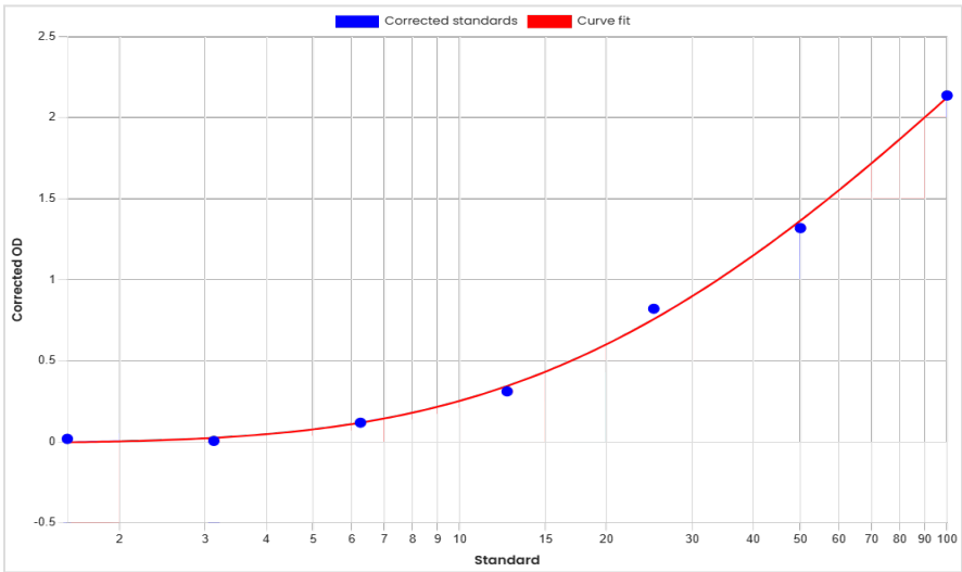
Standard curve anti-ASK8007 antibodies (ADA) ELISA 60467 [ng/mL]
