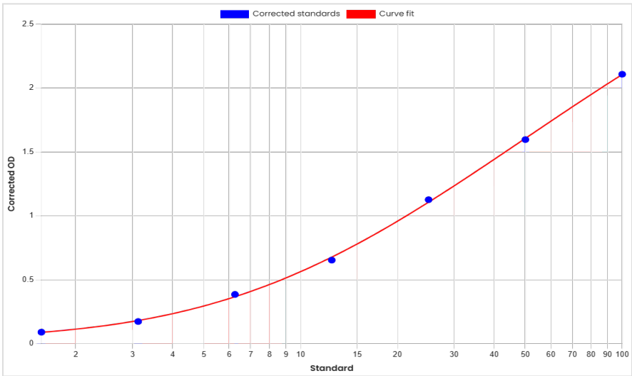
Standard curve anti-BHQ880 antibodies (ADA) ELISA 60457 [ng/mL]
