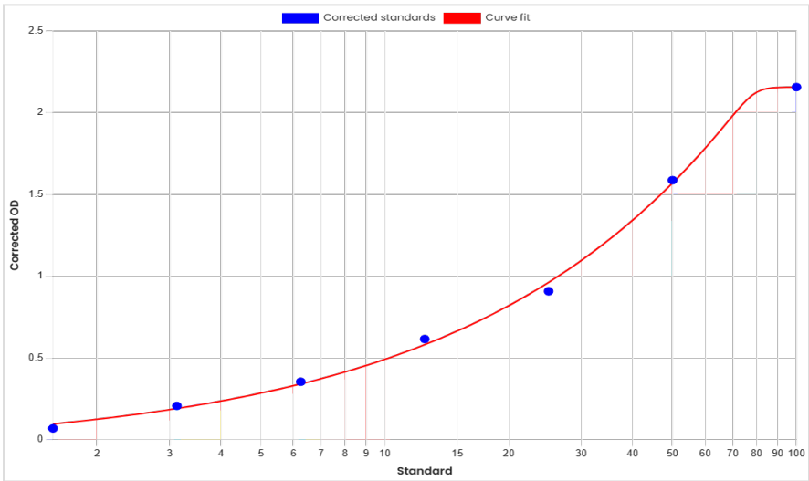
Standard curve anti-Etokimab antibodies (ADA) ELISA 60381 [ng/mL]
