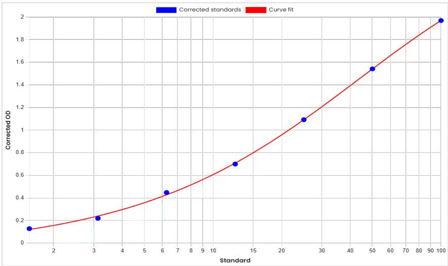
Standard curve anti-Landogrozumab antibodies (ADA) ELISA 60371 [ng/mL]
