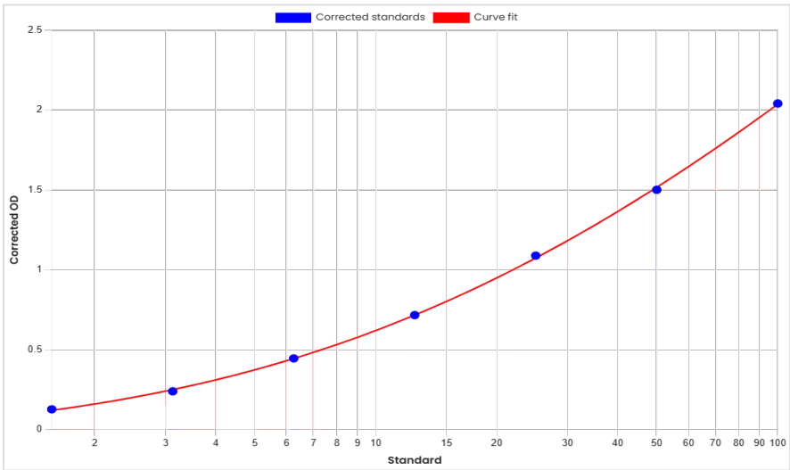
Standard curve anti-Iscalimab antibodies (ADA) ELISA 60353 [ng/mL]
