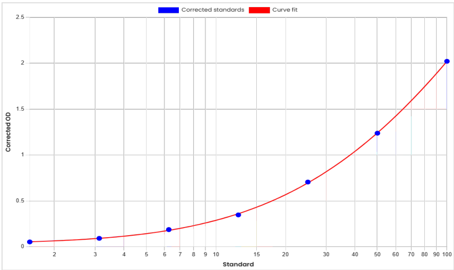
Standard curve anti-Onvatilimab antibodies (ADA) ELISA 60344 [ng/mL]
