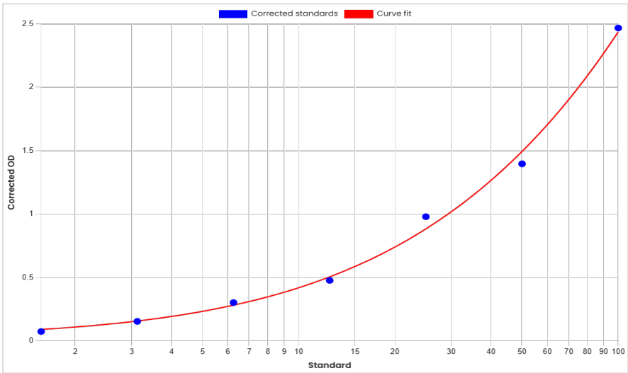
Standard curve anti-Peresolimab antibodies (ADA) ELISA 60315 [ng/mL]
