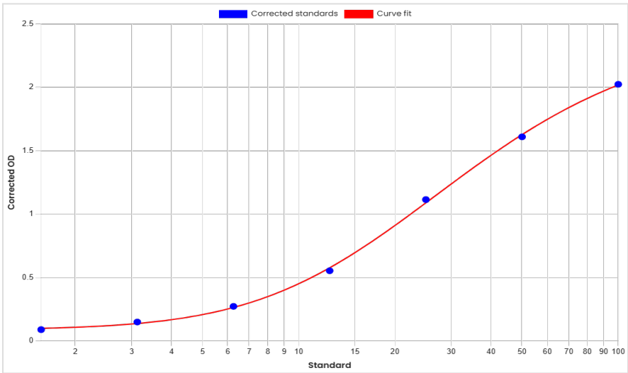
Standard curve anti-Tisotumab antibodies (ADA) ELISA 60261 [ng/mL]
