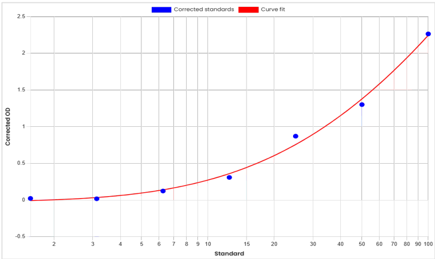
Standard curve anti-Gatralimab antibodies (ADA) ELISA 60242 [ng/mL]
