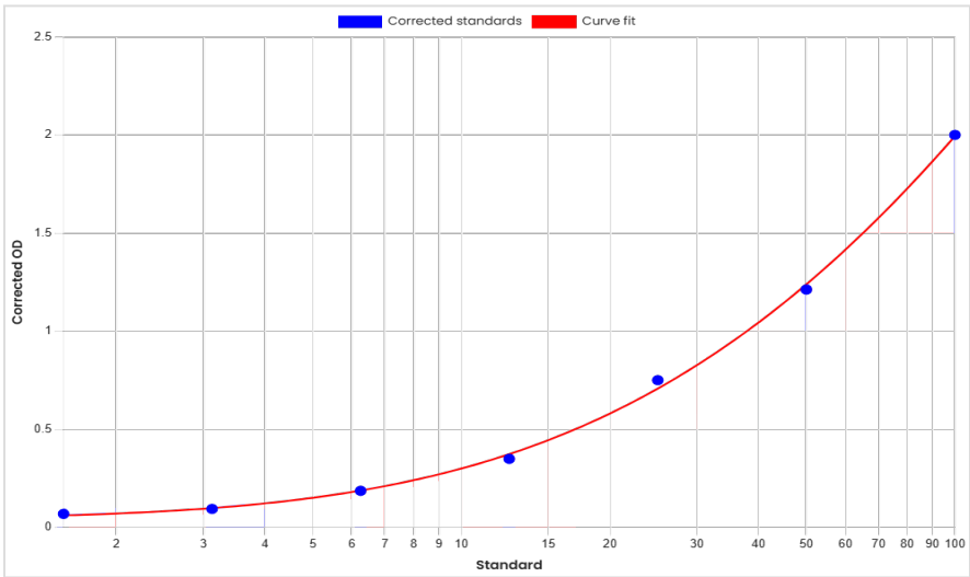
Standard curve anti-Zolbetuximab antibodies (ADA) ELISA 60197 [ng/mL]
