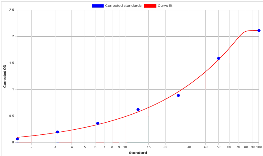
Standard curve anti-Leronlimab antibodies (ADA) ELISA 60178 [ng/mL]
