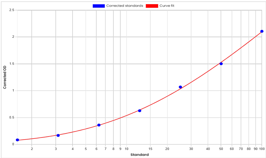
Standard curve anti-Quisovalimab antibodies (ADA) ELISA 60175 [ng/mL]
