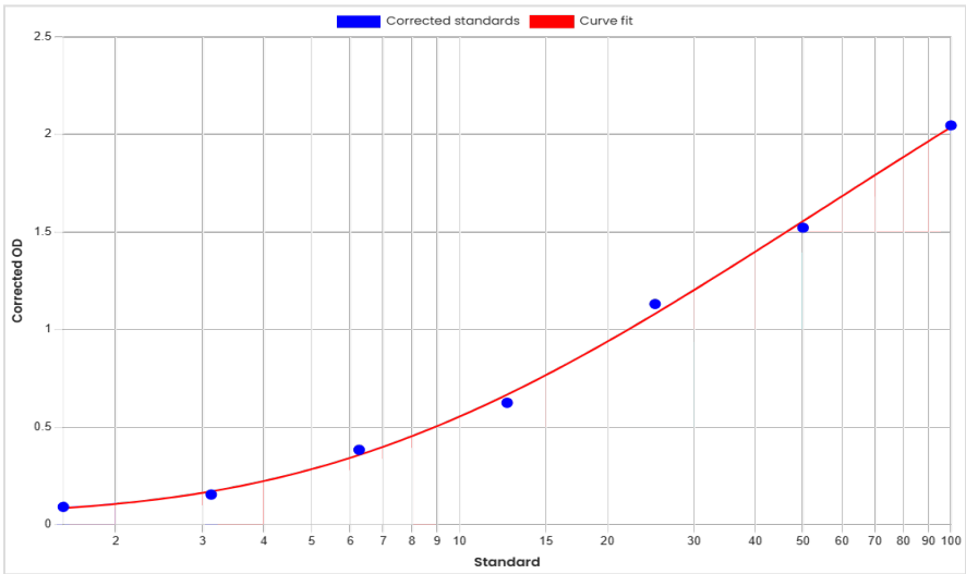
Standard curve anti-CC-90002 antibodies (ADA) ELISA 60168 [ng/mL]
