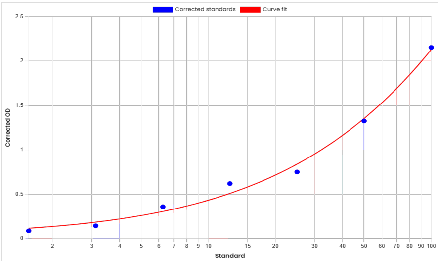
Standard curve anti-Socazolimab antibodies (ADA) ELISA 60166 [ng/mL]
