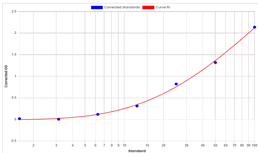
Standard curve anti-Sibrotuzumab antibodies (ADA) ELISA 60156 [ng/mL]
