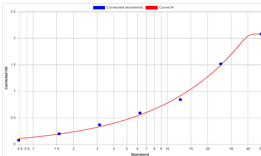
Standard curve Etanercept ELISA 60069 [ng/mL]
