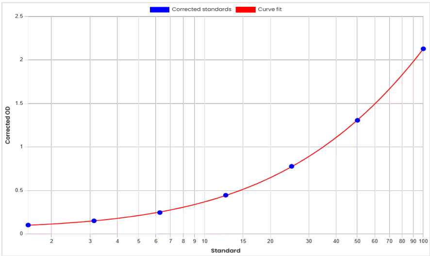
Standard curve anti-Guselkumab antibodies (ADA) ELISA 60056 [ng/mL]
