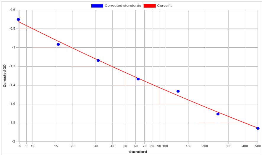
Standard curve Rat AngI-7 (Angiotensin 1-7) ELISA Kit 60043 [pg/mL]
