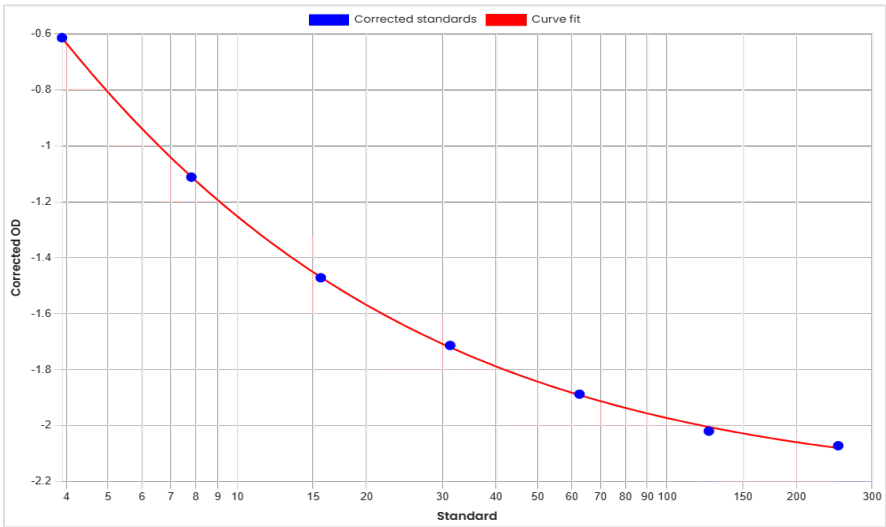
Standard curve Human Anti-Trastuzumab Neutralizing Antibody ELISA Kit 60035 [ng/mL]
