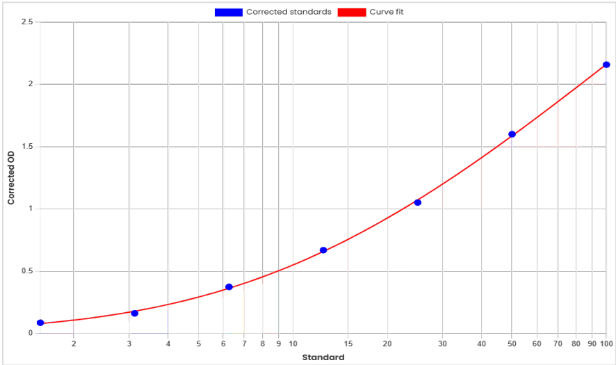
Standard curve anti-Ustekinumab antibodies (ADA) ELISA 60026 [ng/mL]
