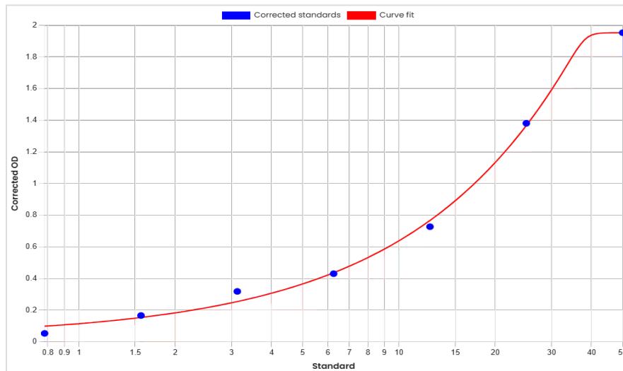
Standard curve anti-Rituximab antibodies (ADA) ELISA 60022 [ng/mL]
