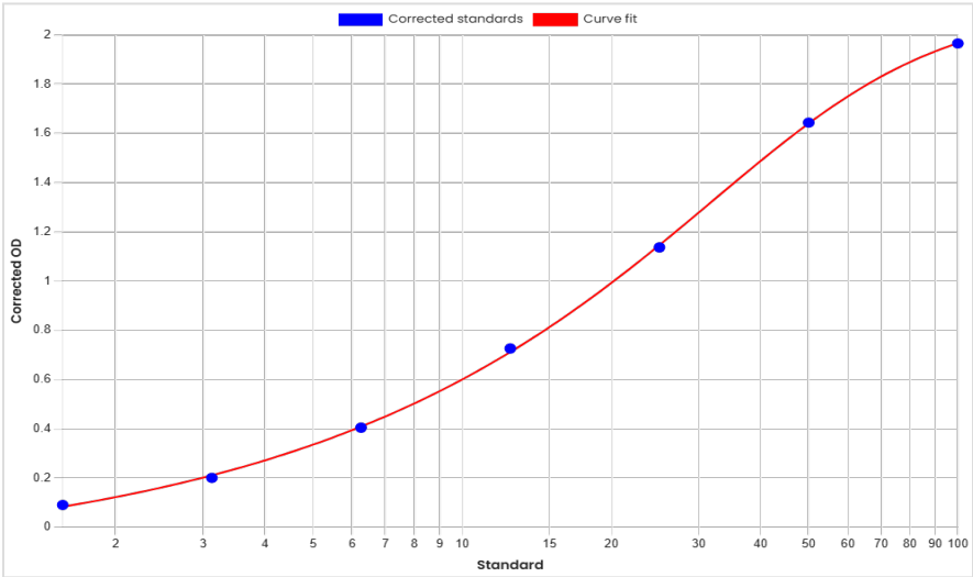
Standard curve dupilumab ELISA 60017 [ng/mL]
