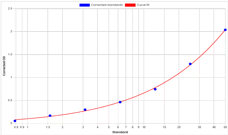
Standard curve Pertuzumab ELISA 60012 [ng/mL]
