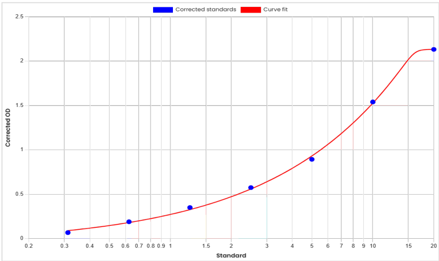
Standard curve anti-Golimumab antibodies (ADA) ELISA 60003 [ng/mL]
